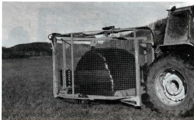
Two rolls of plastic swing around bale, wrapping it tightly in plastic as tractor backs up, rolling bale along ground.
