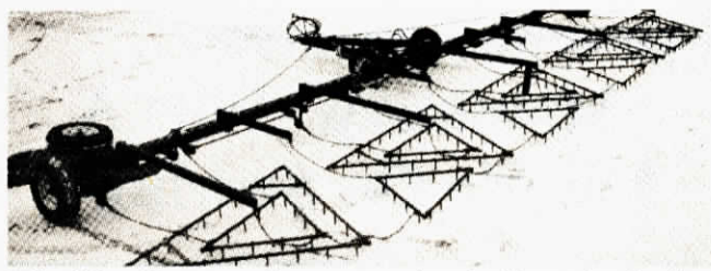
"They'll handle a tremendous amount of trash without plugging," says manufacturer.
