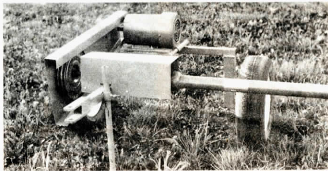
Electric pto handles 8 in. augers up to 60 ft. long.
