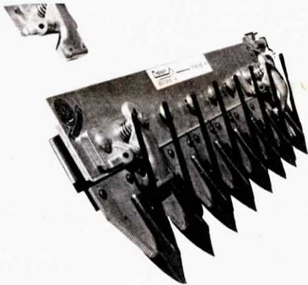
"Slobber Stoppers" plastic fingers glue to top of each sickle guard.
