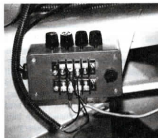
"Junction box" mounts on side of tractor, eliminating the jumble of wires on battery.
